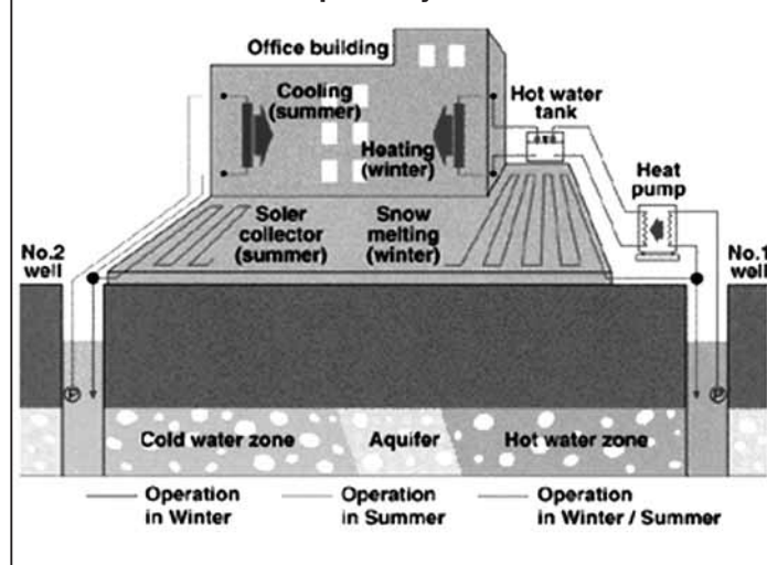
Figure 3: Aquifer System
