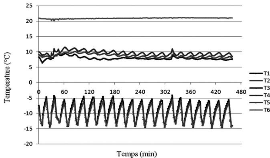
Figure 2. Cool-down and warm-up characteristics of the refrigerator.
