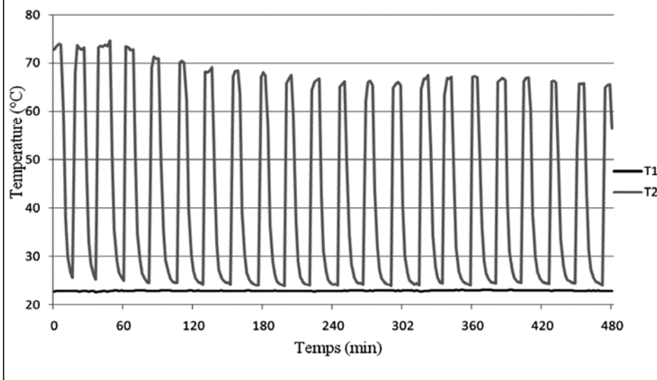
Figure 1. Shows the variation of the compressor body temperature of 50 Hz sinusoidal AC. It can be seen that the compressor body temperature goes through cyclic changes in accordance with the on-off cycle of the refrigerator albeit.
