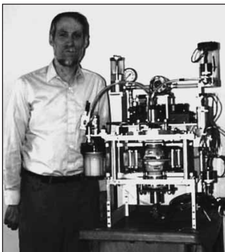
Figure 6. A pioneer of magnetic refrigeration, Dr Carl Zimm, at Astronautics beside the built magnetic refrigerator prototype, which is schematically shown in Figure 5. Printed with permission from Astro-nautics Corporation of America.
