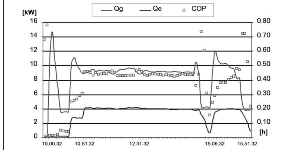
Figure 5. COP, Power supply ( Q_g ) and cooling power ( Q_c ) of Machine D ( T_{g,i} = 80 °C, T_{t,o} = 26 °C).
