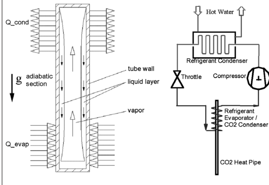
Figure 3: Working principle of a heat pipe (two-phase thermosyphon) and heat pump system layout
