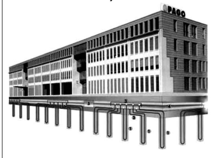
Figure 2: Pile System
