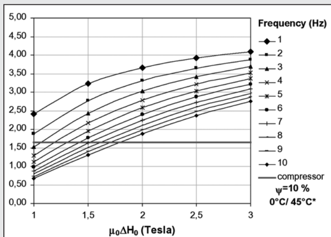
Fig. 1. The coefficient of performance, COP, of a magnetic household refrigerator as a function of the magnetic field density (presented as an induction) and its frequency of operation are shown (from Ref. [2]). The coefficient of performance of the conventional machine naturally shows no dependence on the magnetic field (as such a field is not present in such a device) and, therefore, appears in this figure as a constant.
